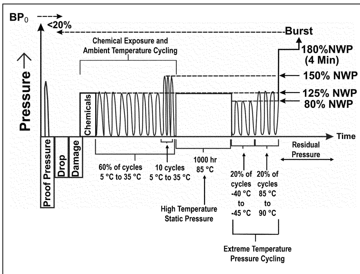
Figure-4: Illustration of the Test for Performance Durability
