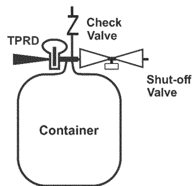
Figure-3: Typical CHSS
