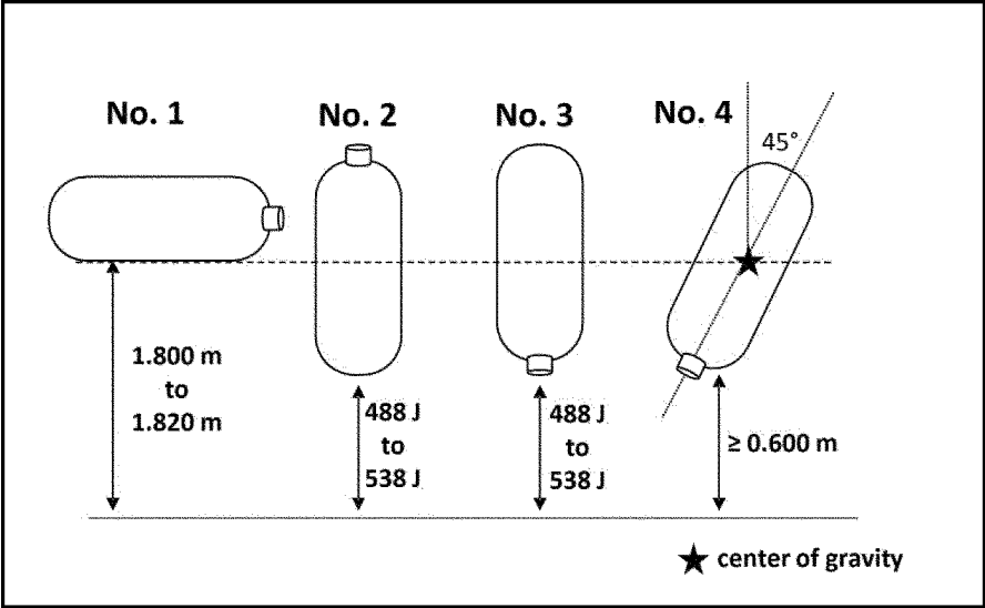
Figure 2. The Four Drop Orientations; (for Illustration Purposes Only)
