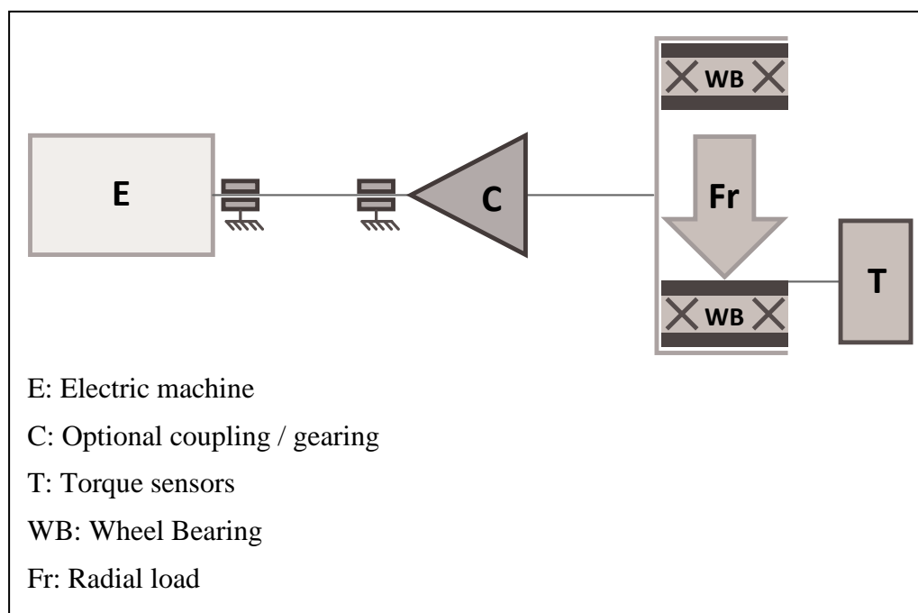
Figure 1. Simplified schematic of the test set-up
