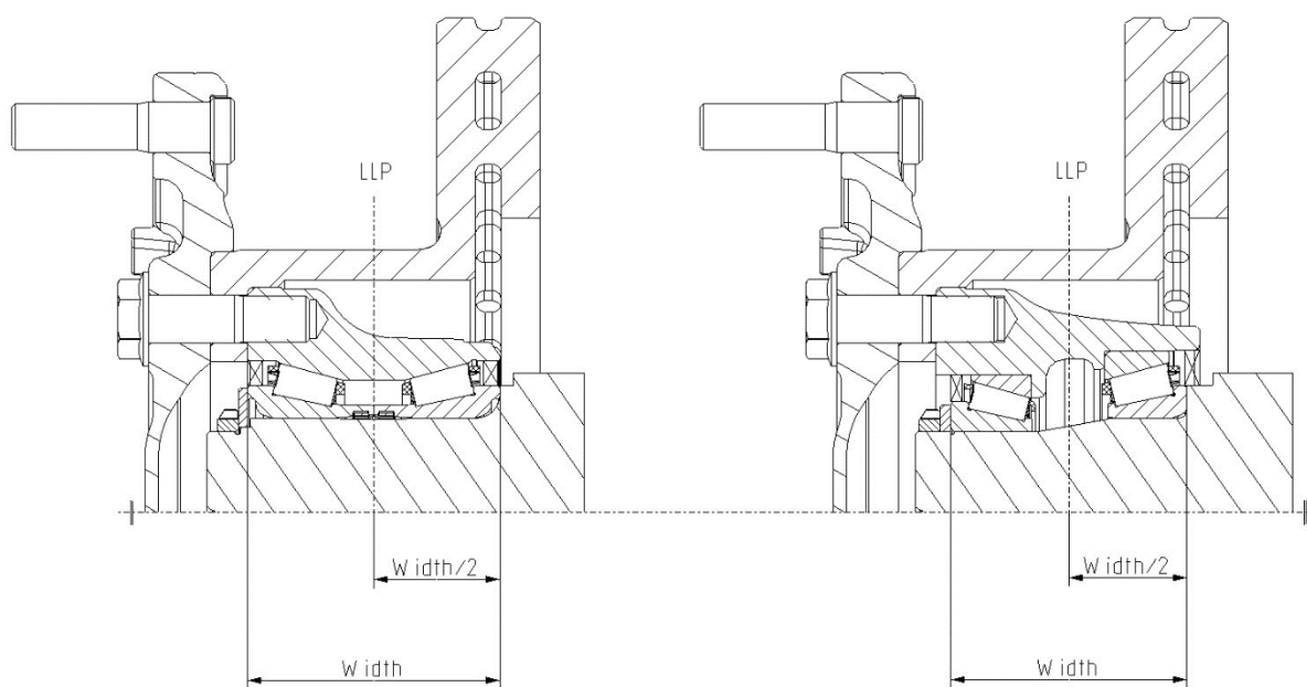
Figure 2 – Determination of Load Line Position
