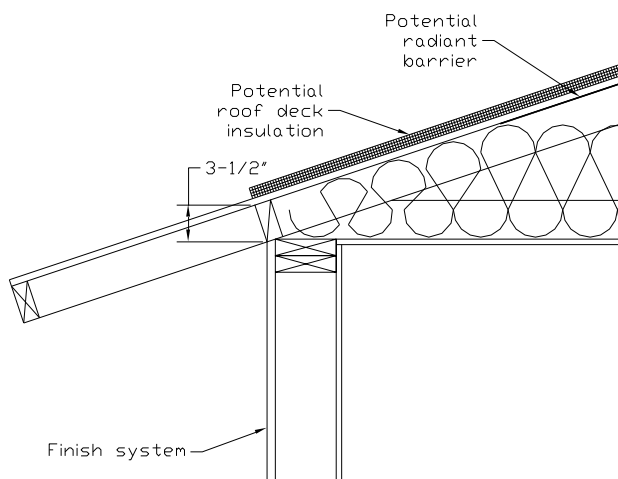
Figure 181818 17: Section at Attic Edge with Standard Truss
