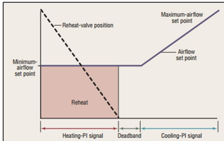
Figure 888 9: Single Maximum VAV Box Control
