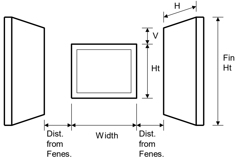
Figure 1616 1615: Sidefin Dimensions
