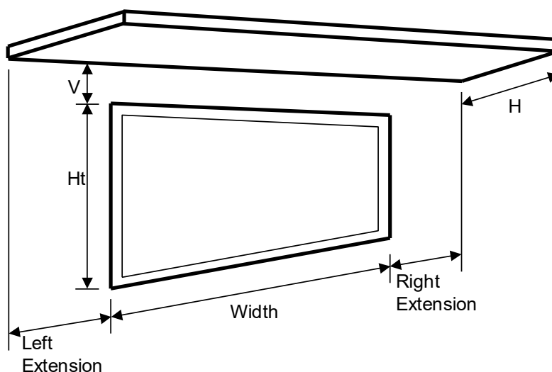
Figure 15151514 1514: Overhang Dimensions
