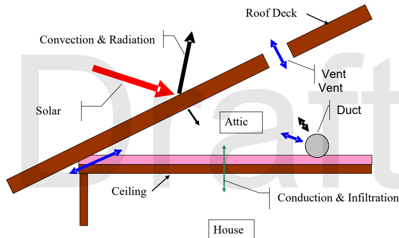
Figure 17 16 17: Attic Model Components
