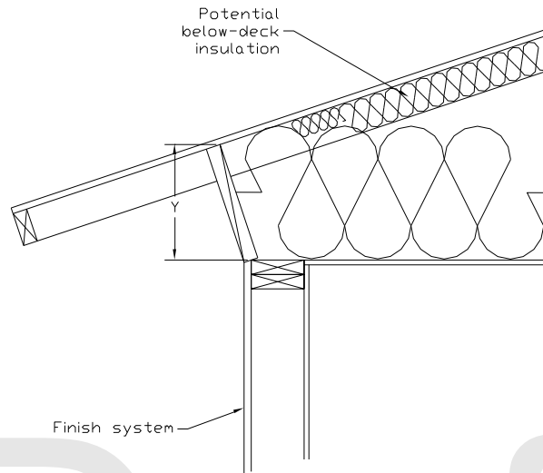
Figure 19 19 18 : Section at Attic Edge with a Raised Heel Truss
