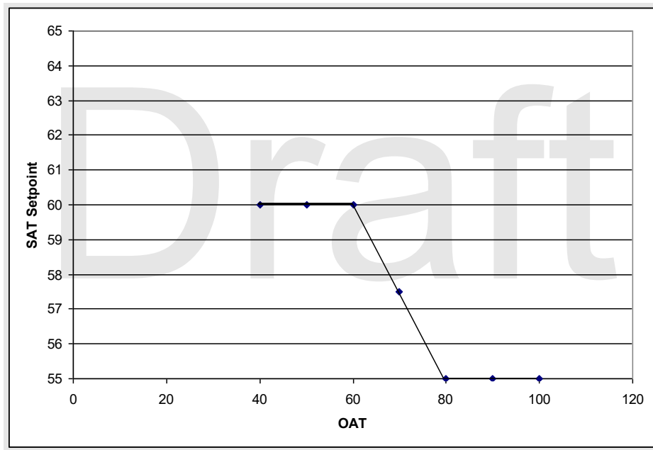
Figure 101011: SAT Cooling Setpoint Reset Based on Outdoor Air Temperature (OAT)
