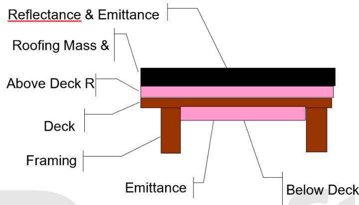
Figure 20202019 Components of the Attic Through Roof Deck
