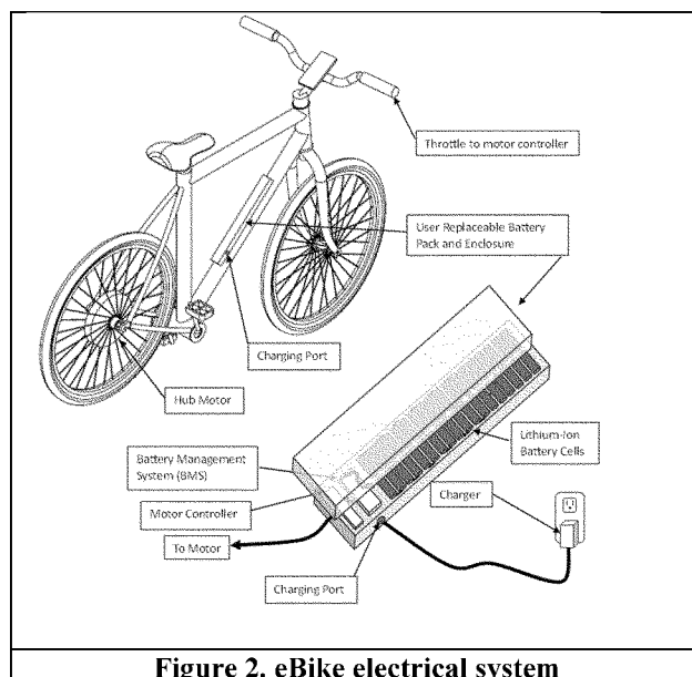
Figure 2. eBike electrical system
